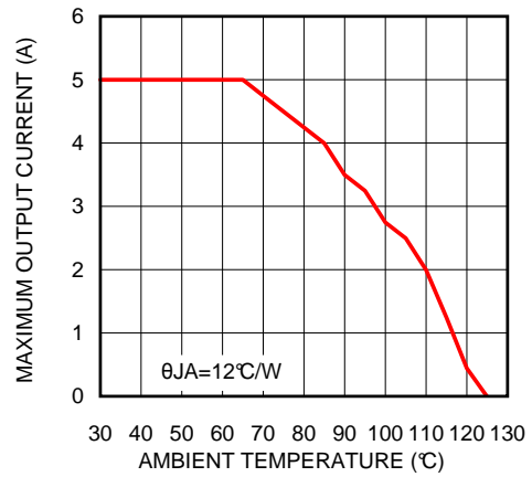
Thermal Derating Curve V_{IN} = 12V V_{OUT} = 5.0V
